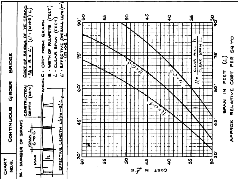
Fig. 263.—Cost of Continuous Girder Bridges.
